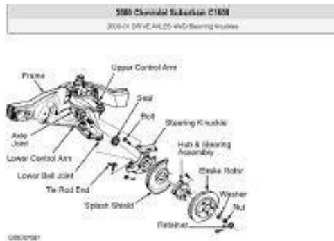
Fig. 1. Exploded View Of Hub & Steering Knuckle Assembly ("T" Series Shows "K" & "U" Series Are Similar) Courtesy of GENERAL MOTORS CORP.
